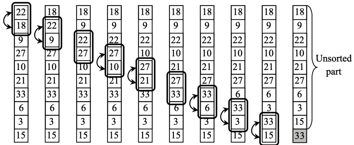
Fig.2.1. First pass of bubble sort
