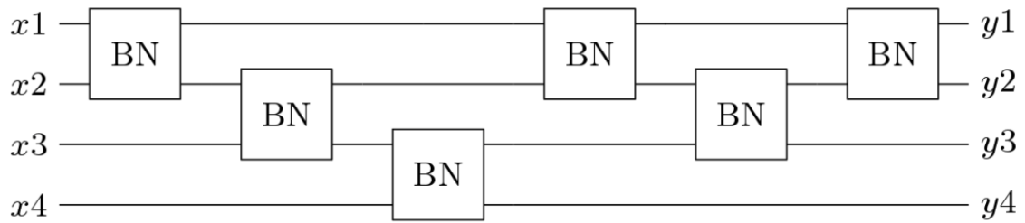
Figure 1: Bubble Sort for n=4
